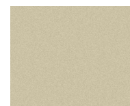
Kubanite
